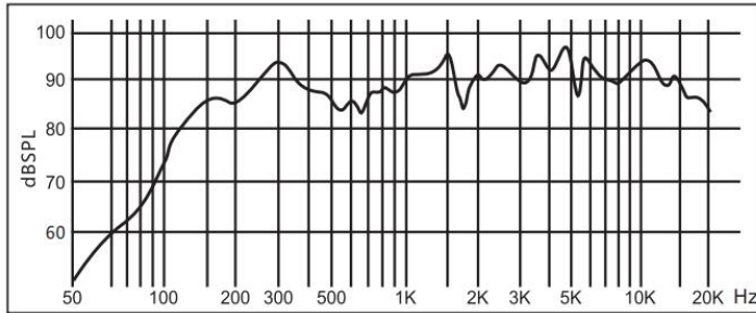
Frequency Response Characteristic (dB SPL、1W、1m)
